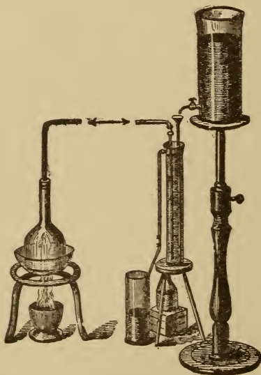
Fig. 107½. MITSCHERLICH'S APPARATUS FOR THE DETERMINATION OF PHOSPHORUS.
